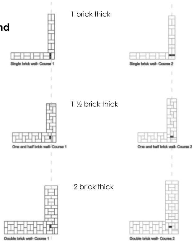
C8 Hazard Resistant Features for Foundation and Plinth NDMA Unnati PIC
