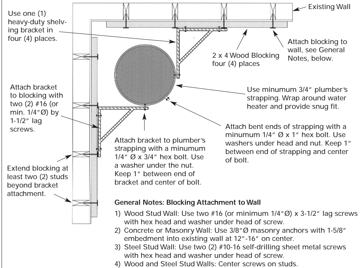
Figure 12: Corner Wall Configuration
