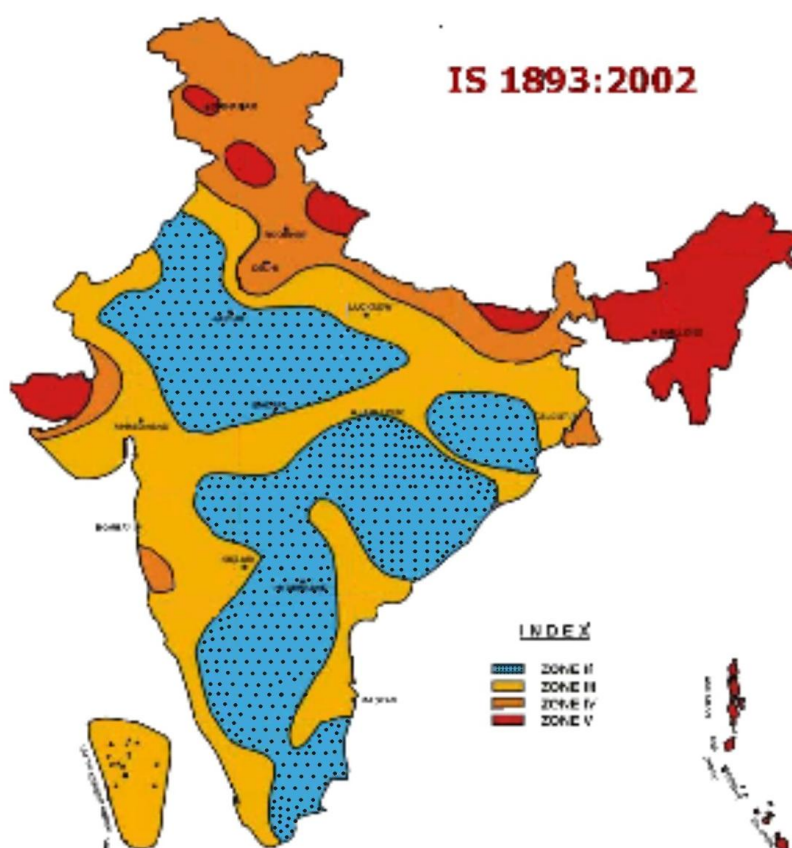
Figure 1: Seismic Zone Map of India based on IS 1893 (1): 2002
